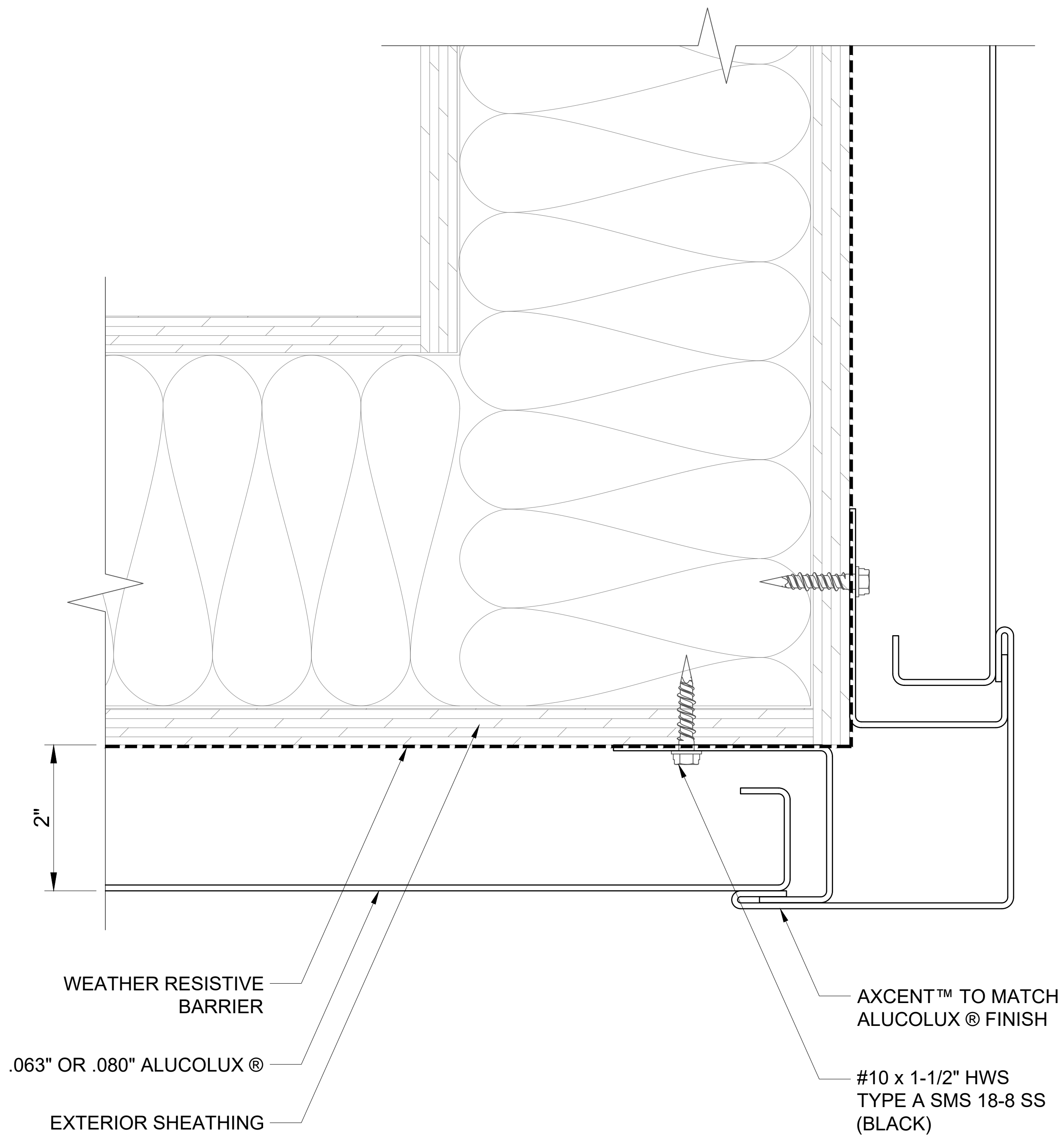
306 OUTSIDE CORNER SCALE: 3" = 1' - 0"
