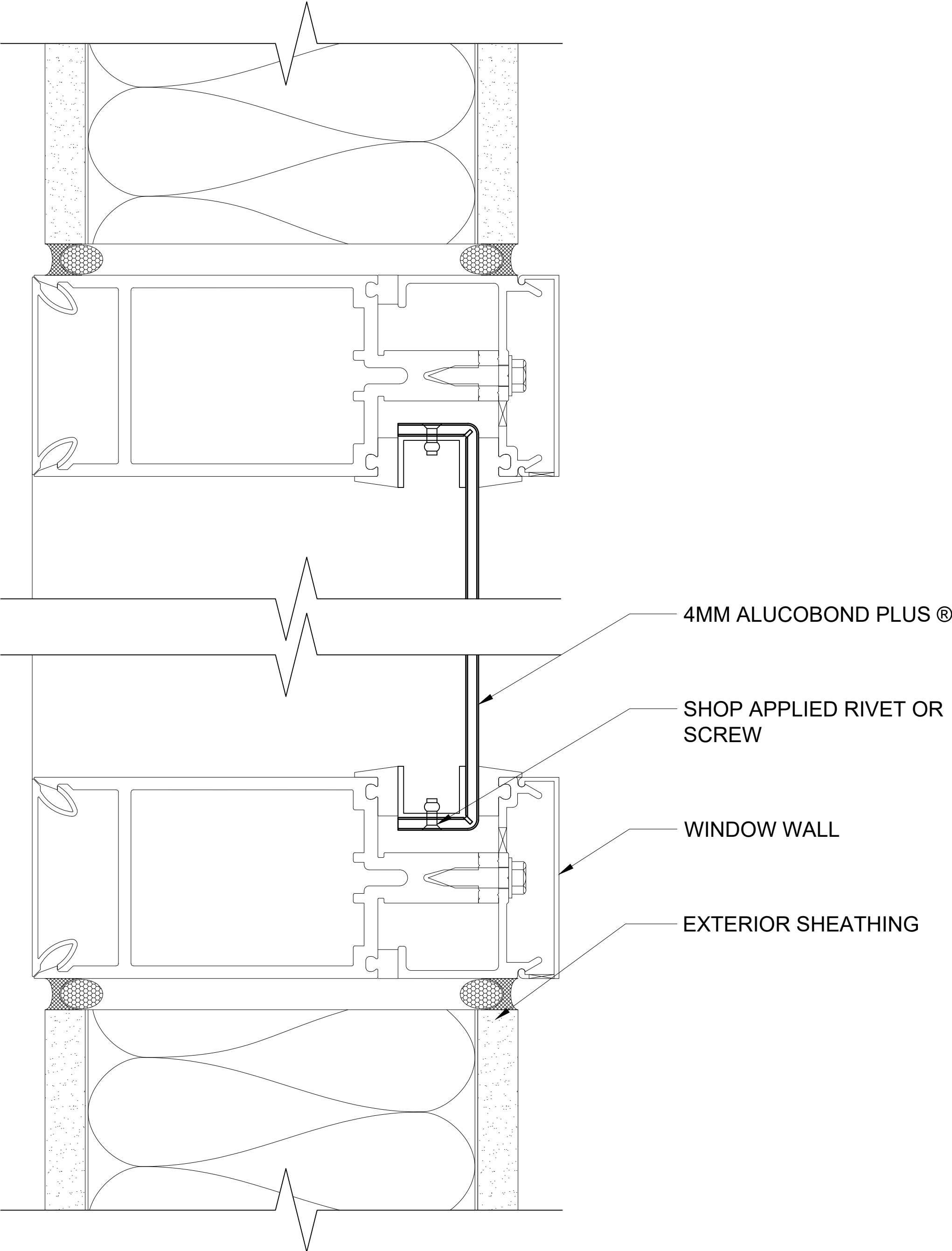
220 FACE CAPTURED CURTAIN WALL SCALE: 3" = 1' - 0"
