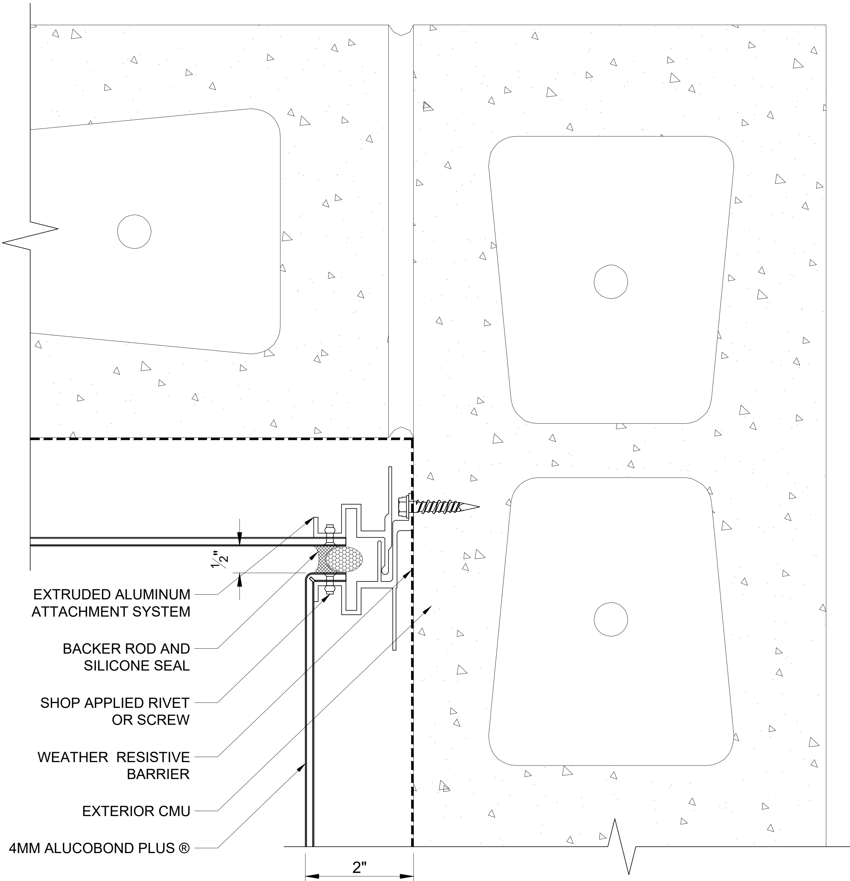
310 INSIDE CORNER - PLAN VIEW SCALE: 3" = 1' - 0"
