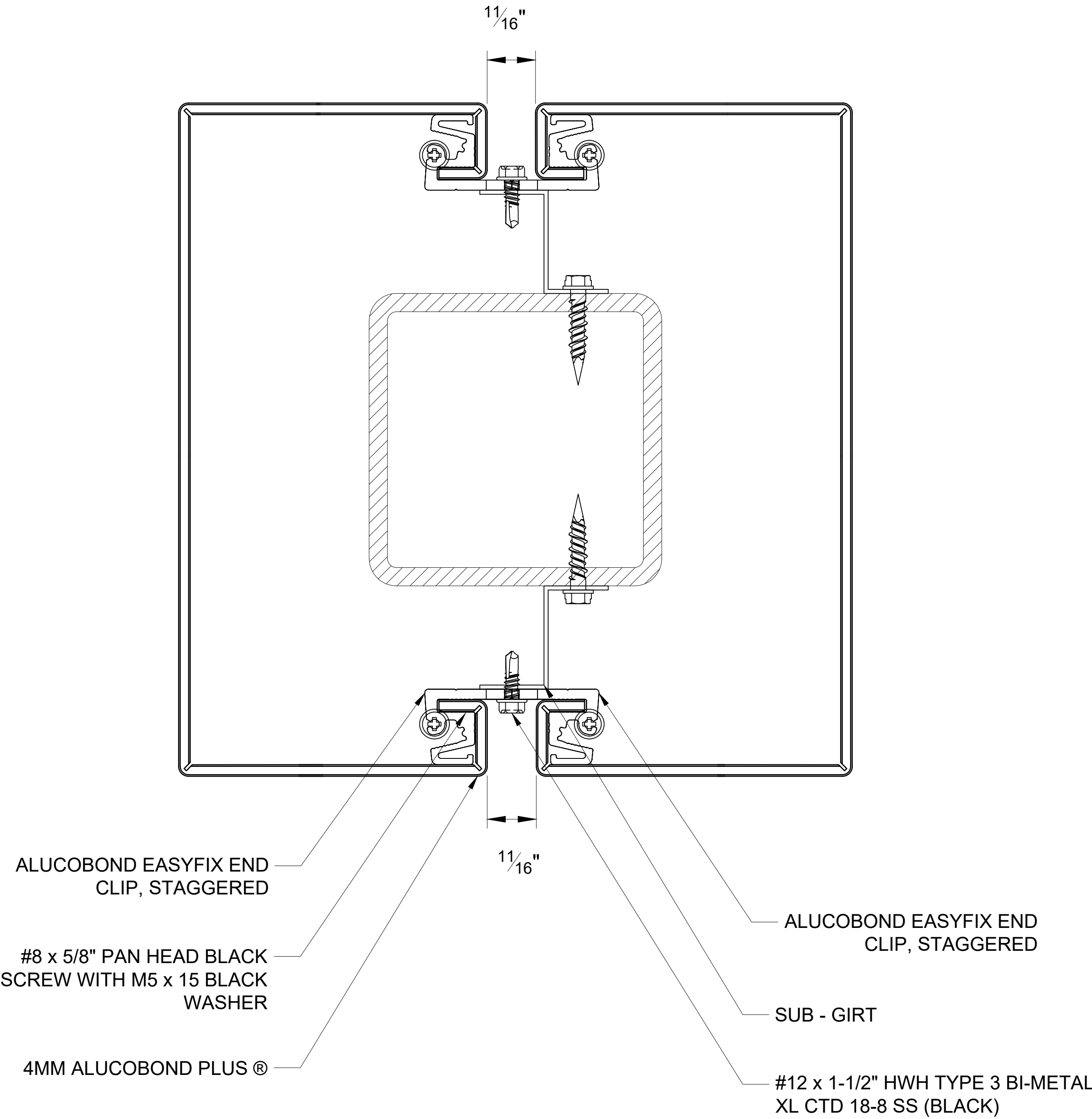
116 SQUARE COLUMN COVER SCALE: 3" = 1' - 0"
