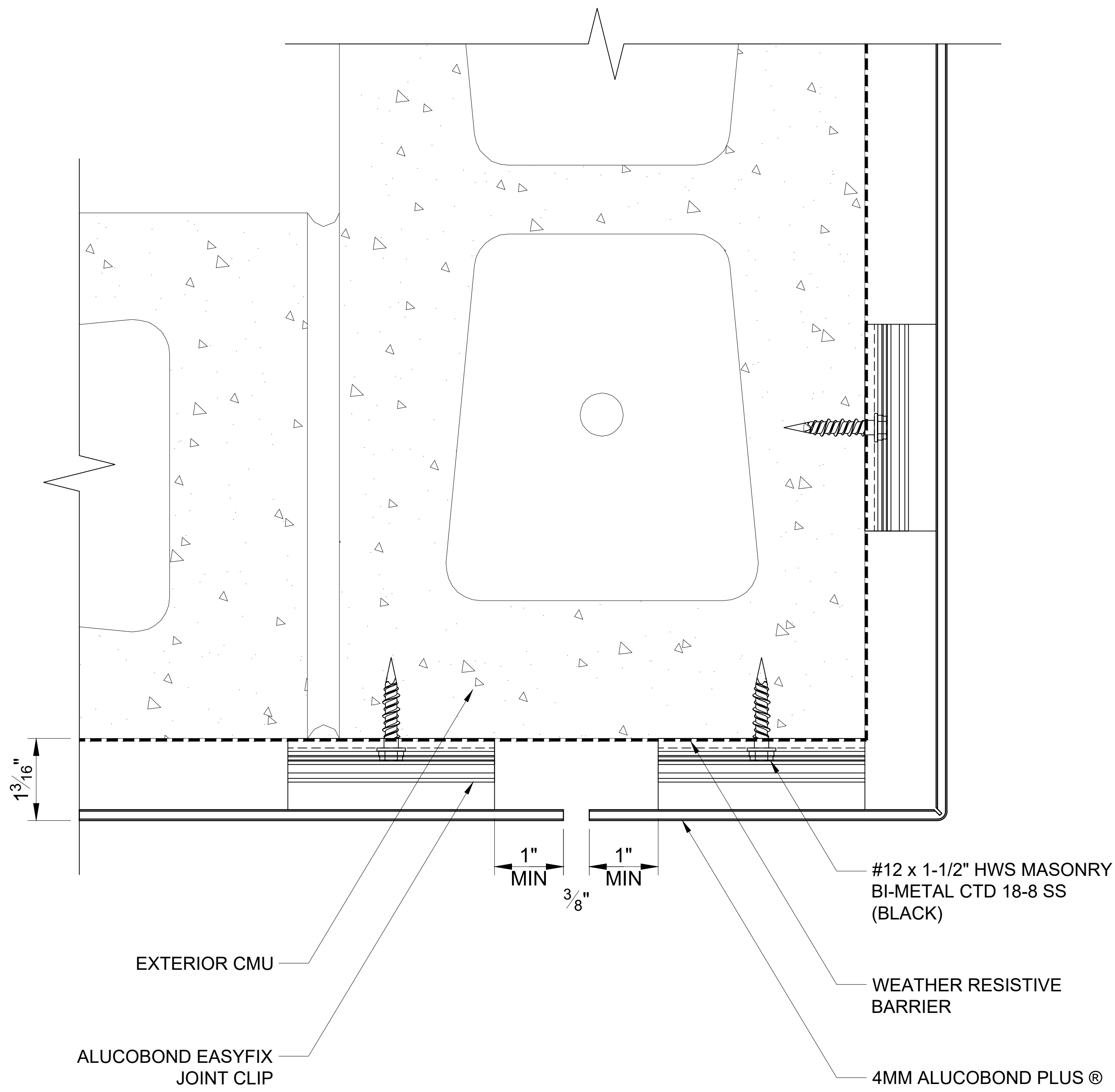
405 OUTSIDE CORNER SCALE: 3" = 1' - 0"
