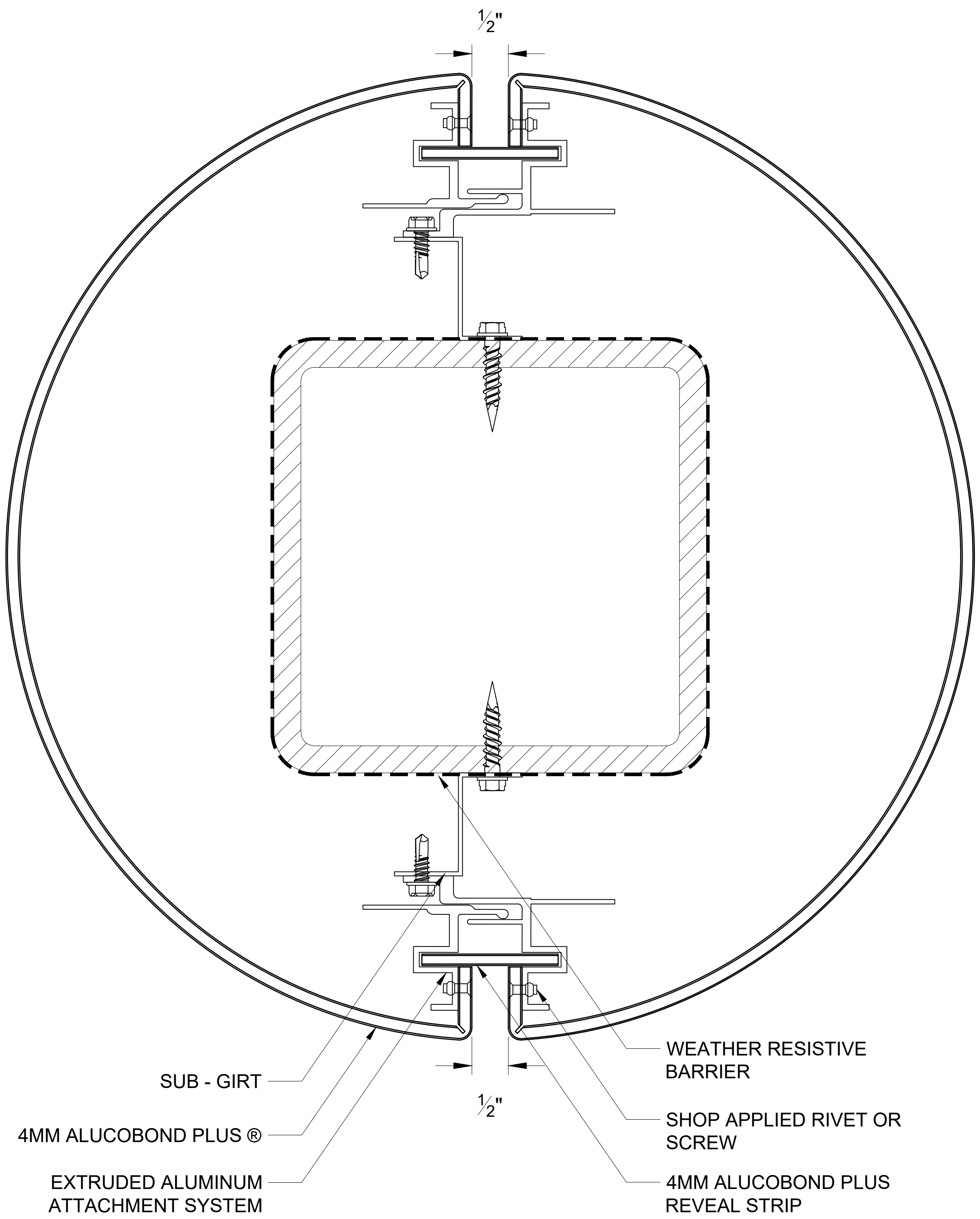
123 RADIUS COLUMN COVER - PLAN VIEW SCALE: 3" = 1' - 0"
