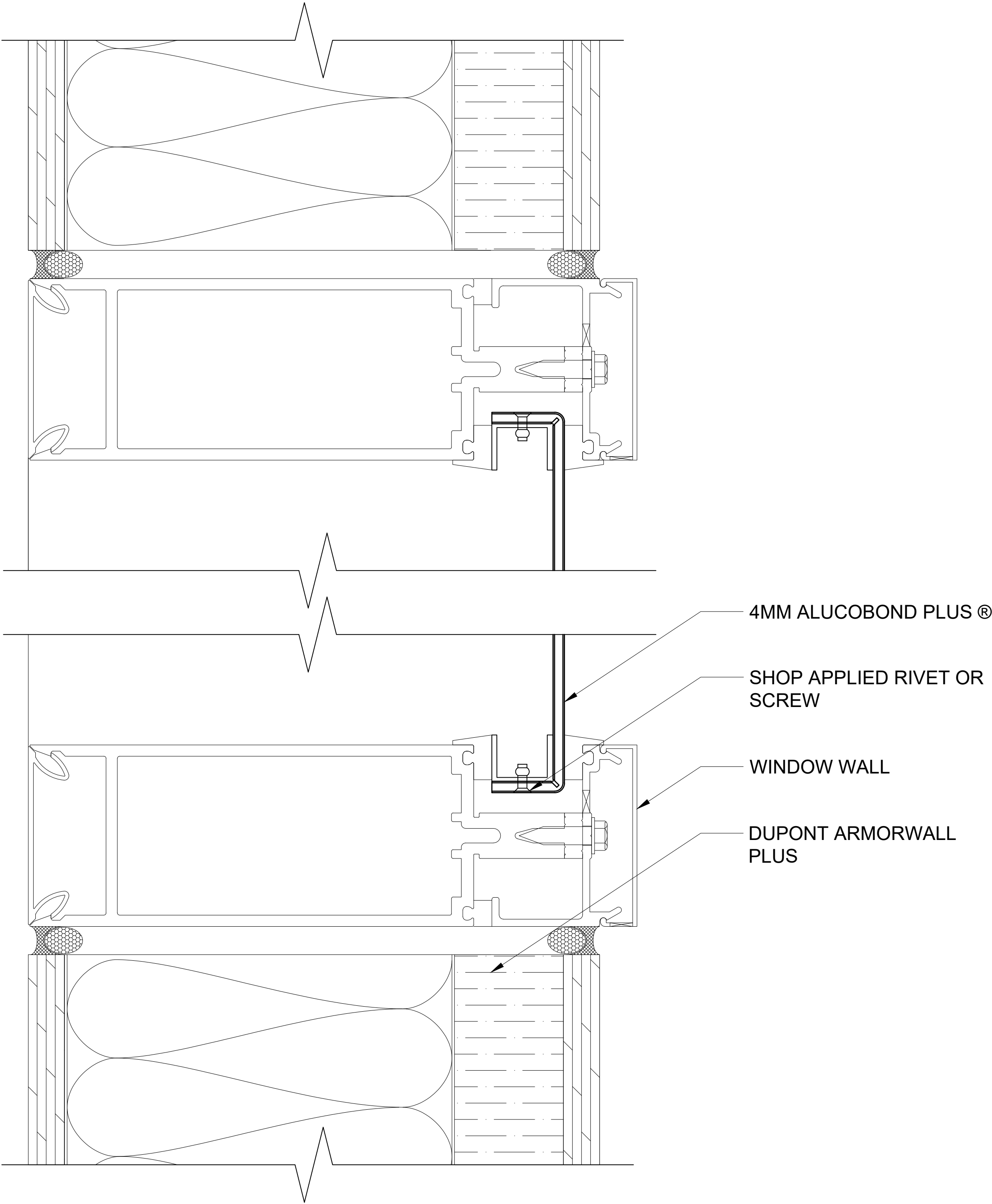
520 FACE CAPTURED CURTAIN WALL SCALE: 3" = 1' - 0"
