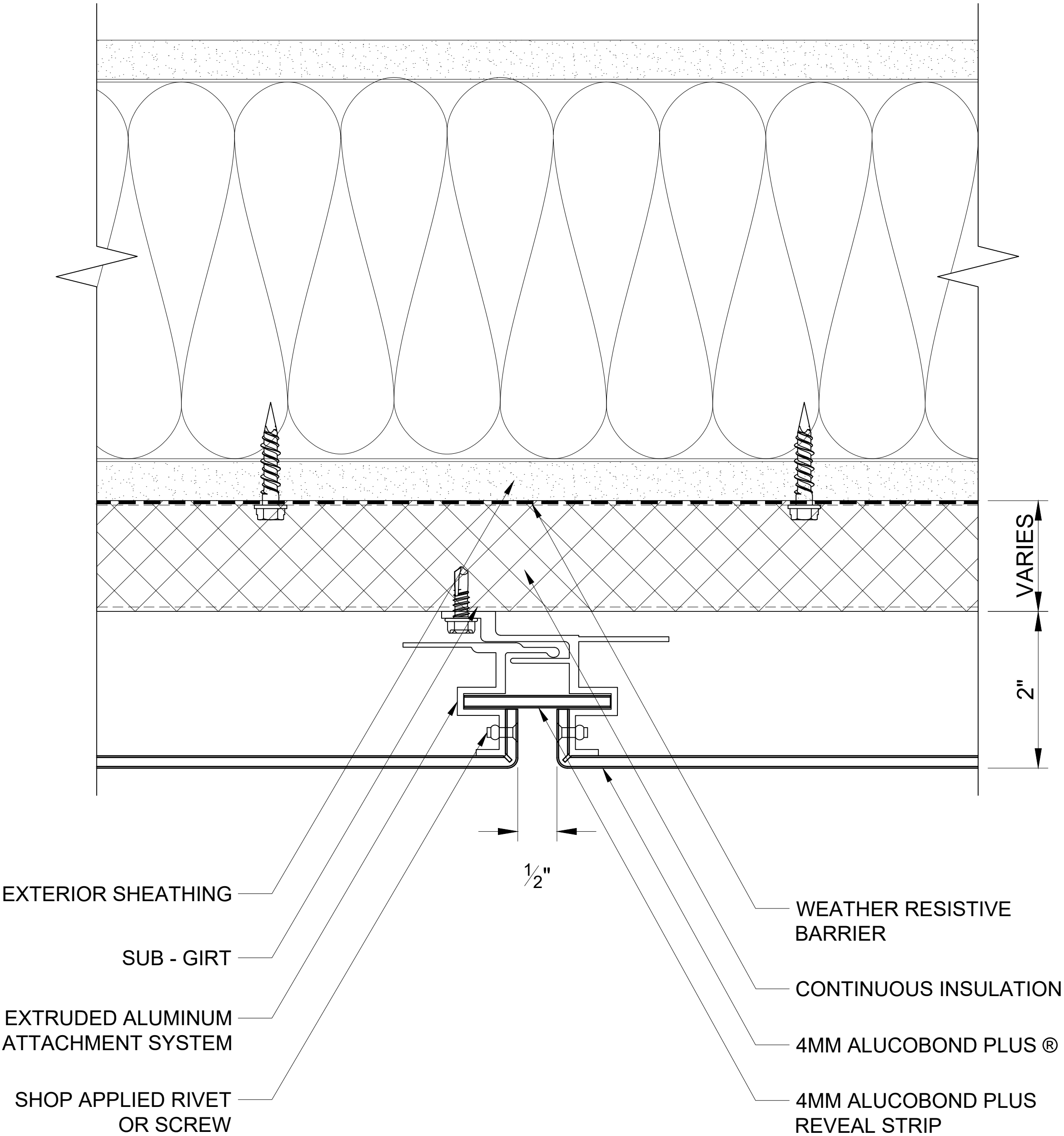
104 VERTICAL JOINT - PLAN VIEW SCALE: 3" = 1' - 0"
