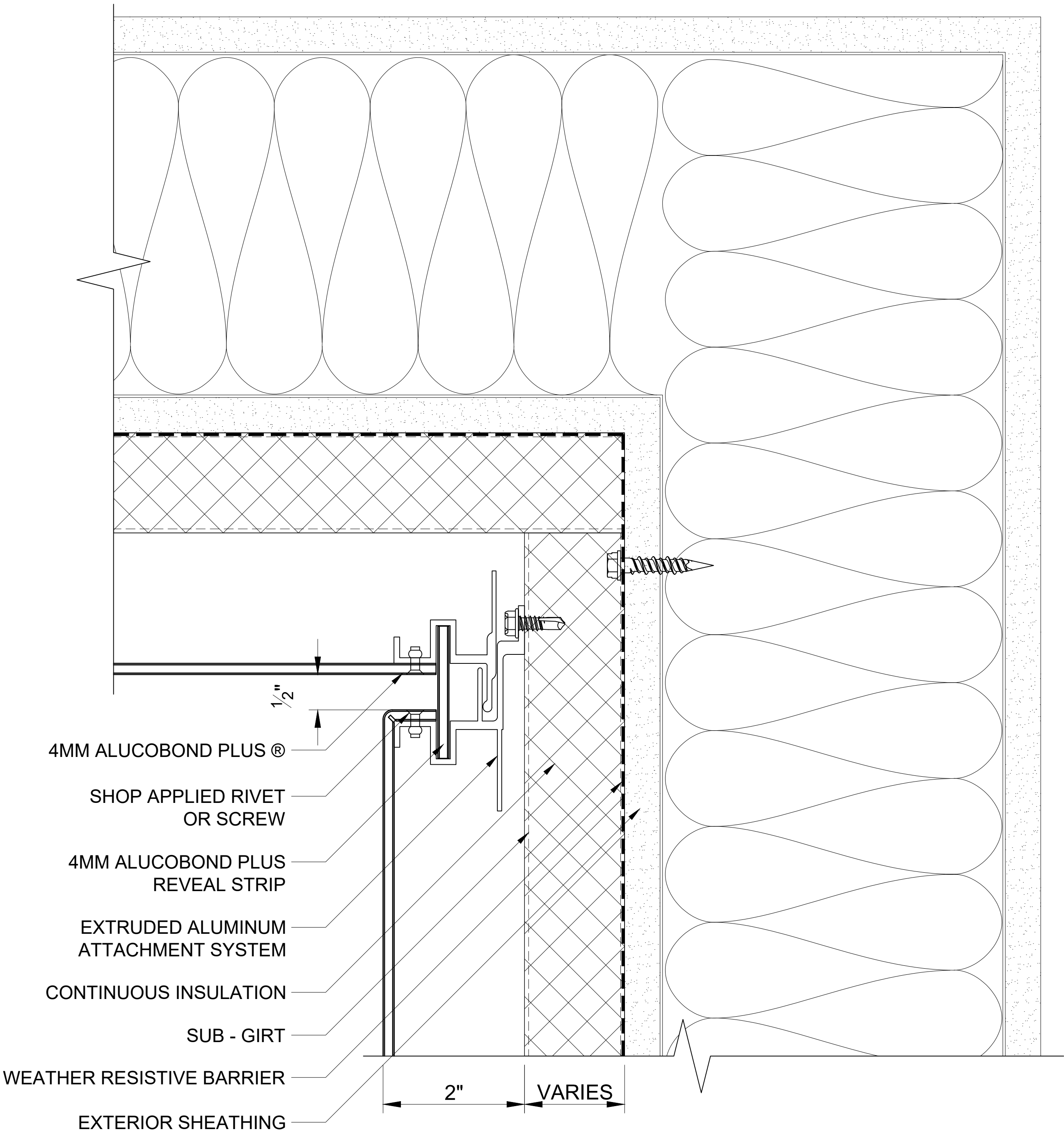
110 INSIDE CORNER - PLAN VIEW SCALE: 3" = 1' - 0"
