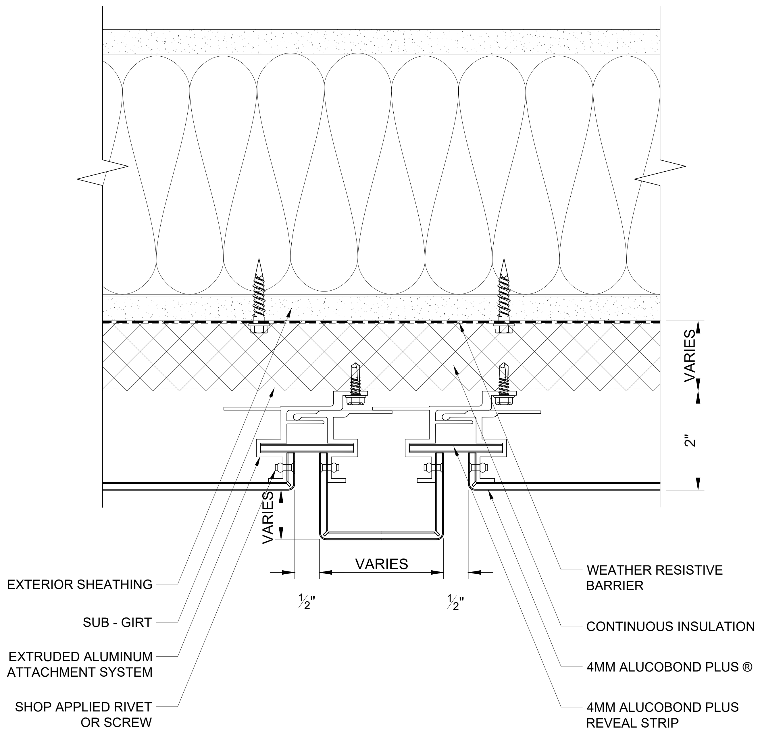
105 PROUD PANEL FIN - PLAN VIEW SCALE: 3" = 1' - 0"
