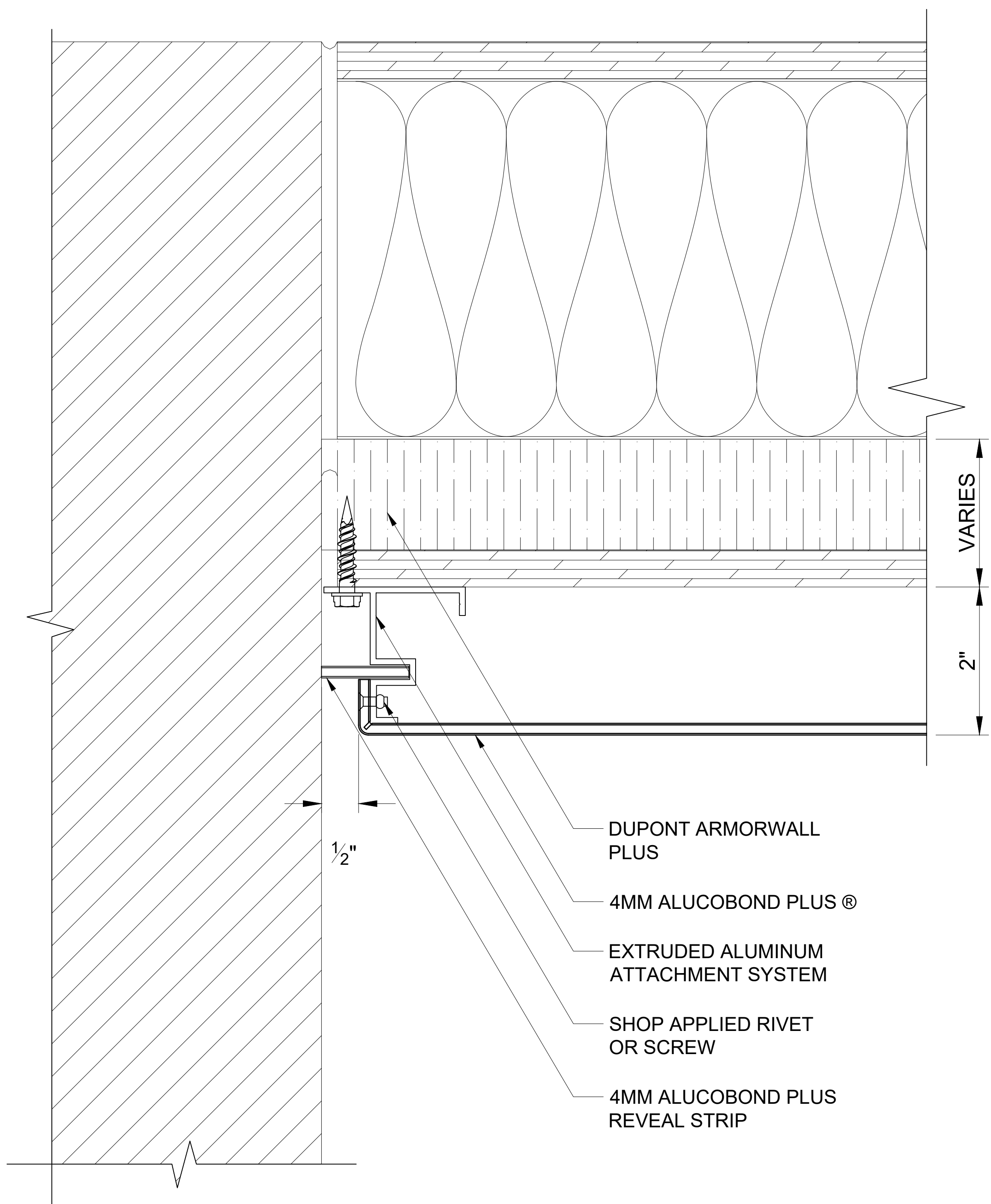
507 END WALL - PLAN VIEW SCALE: 3" = 1' - 0"
